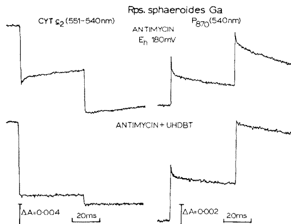
Fig. 2. Double flash kinetics of cyt c_2 and P -870. With antimycin A: Same conditions as for fig. 1A (with antimycin A). Traces are an average of 2. Time between flashes was 46 ms. The instrument response time was 100 \mu s. With antimycin A and UHDBT: As above but UHDBT was added to 40 \mu M.
